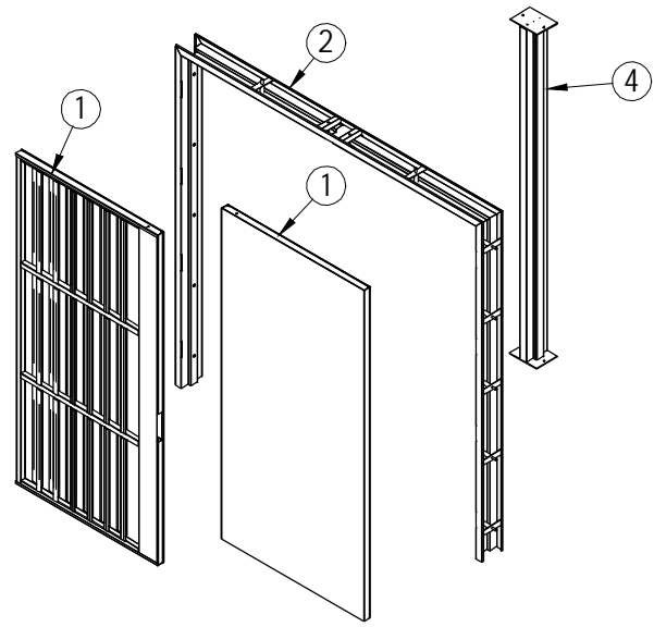
EXPLODED VIEW
