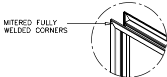
CORNER DETAIL 'B'
