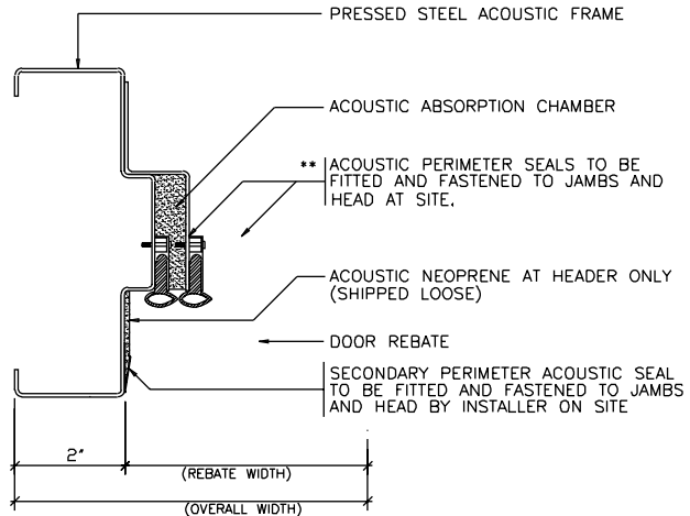
TYPICAL JAMB SECTION
