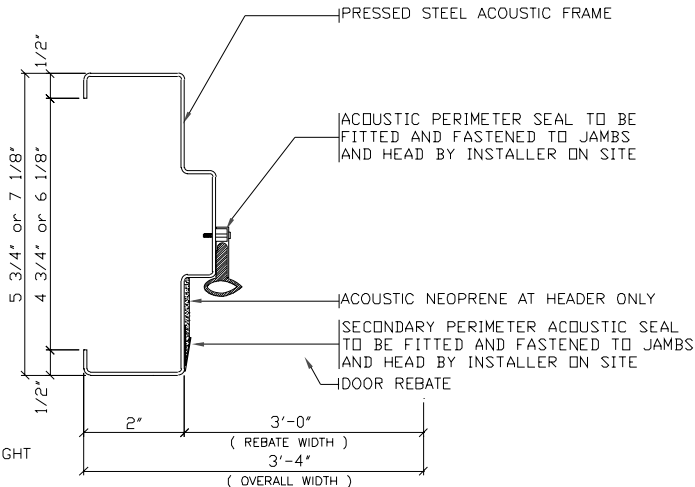
TYPICAL JAMB SECTION
