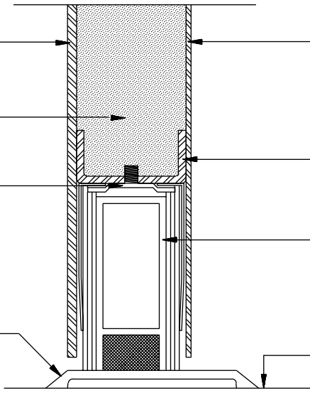
TYPICAL ACOUSTIC DOOR & DOOR BOTTOM - STC 52
