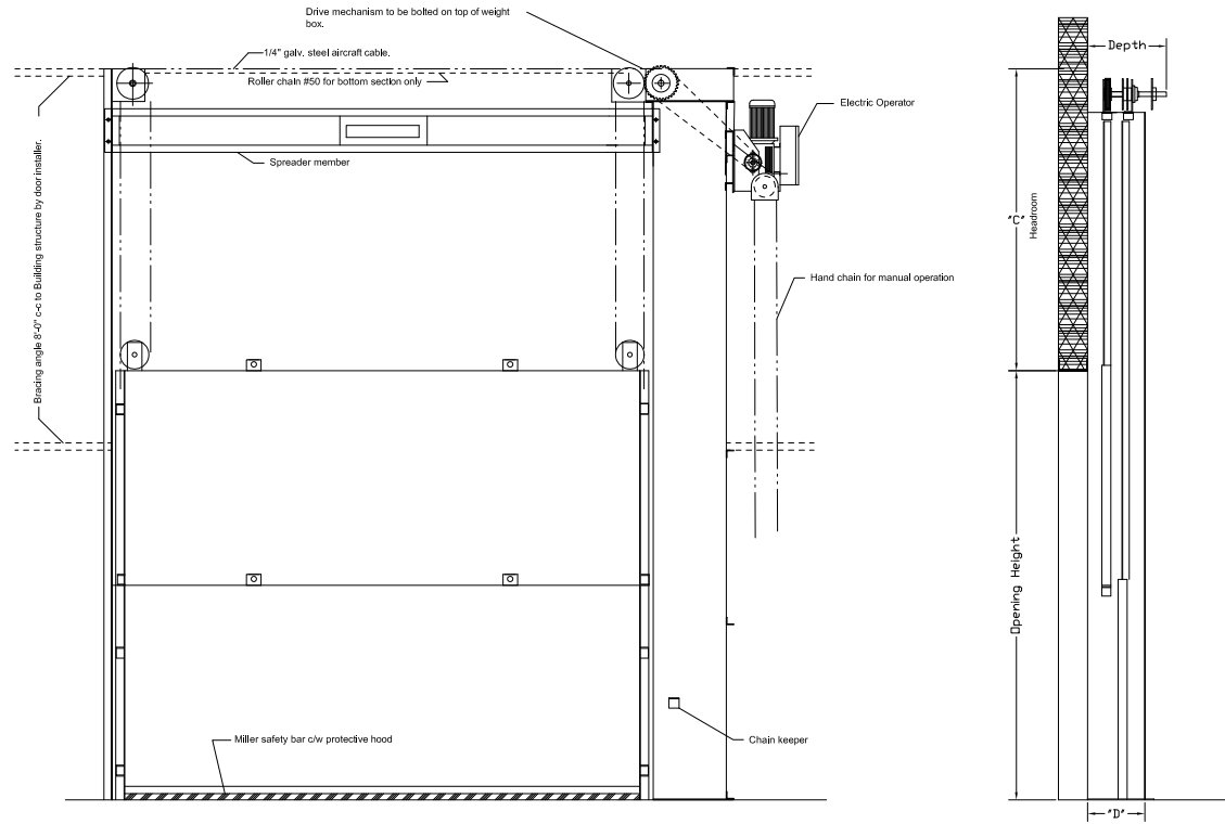
INTERIOR ELEVATION
