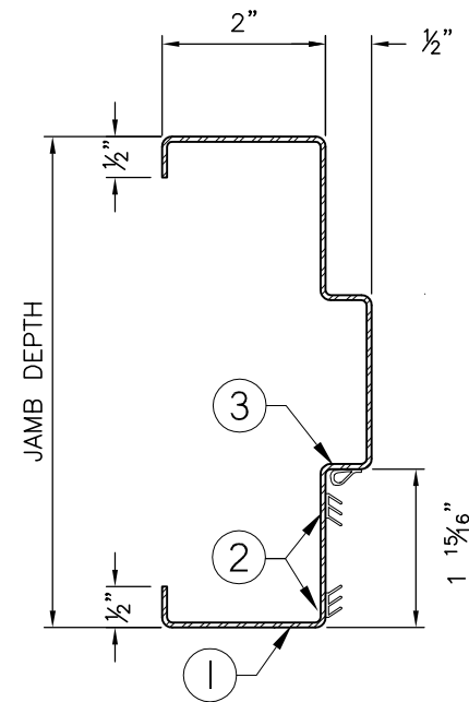
TYPICAL JAMB SECTION
